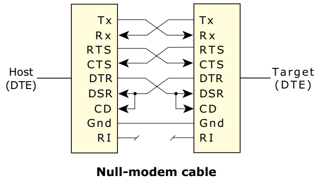
Null-modem cable pinout.
