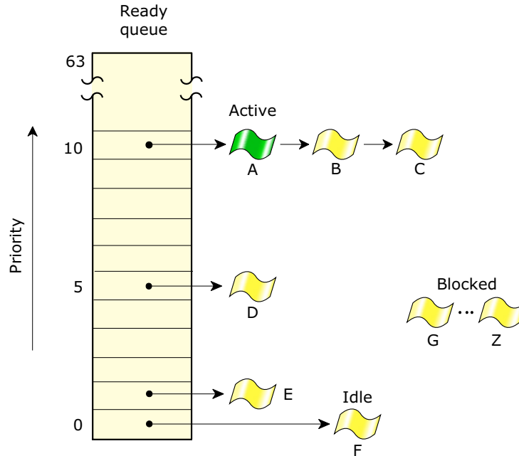
The ready queue for six threads (A-F) that are READY. All other threads (G-Z) are BLOCKED. Thread A is currently running. Thread A, B, and C are at the highest priority, so they'll share the processor based on the running thread's scheduling algorithm.
